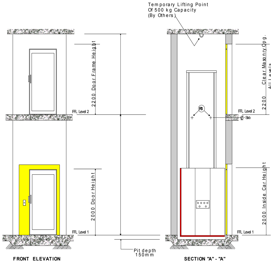
FRONT ELEVATION
