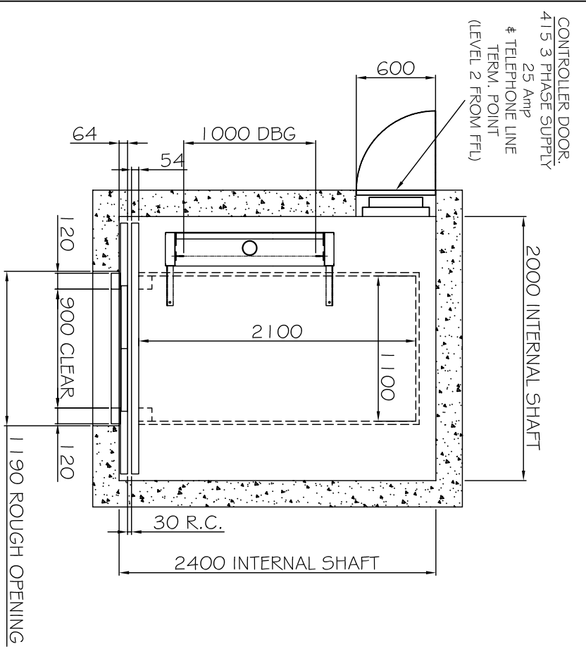
WELL PLAN
