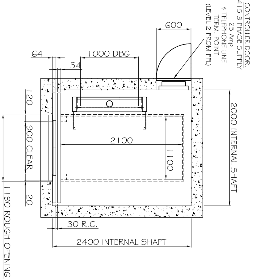
WELL PLAN
